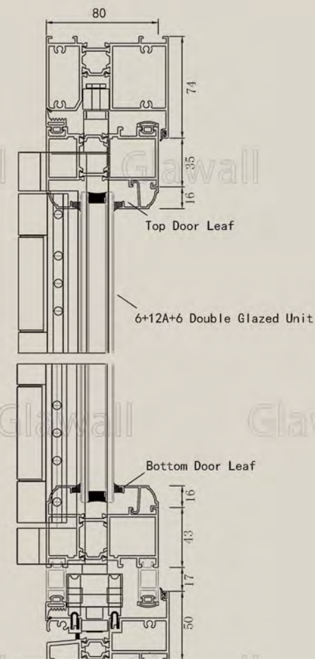
S80 Folding Glass Door | Panel THK: 80mm
