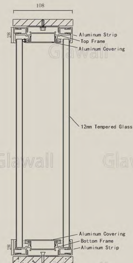
108 Series Frameless Double Glass | Panel THK: 108mm
