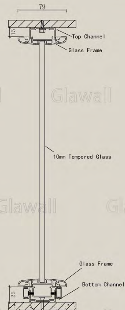
79 Series Single Glass | Panel THK: 79mm
