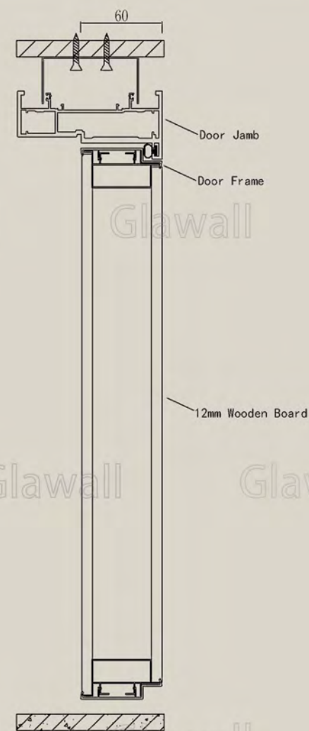
60 Series Wooden Door | Panel THK: 60mm
