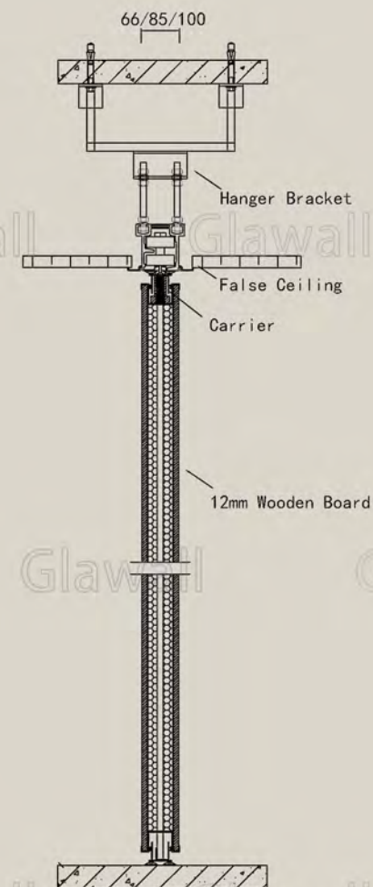
66, 85 100 Series Movable wall | Panel THK: 66, 85, 100mm
