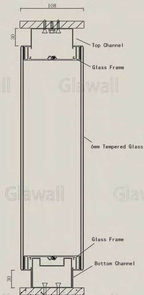
108 Series Hidden Frame Glass | Panel THK: 108mm
