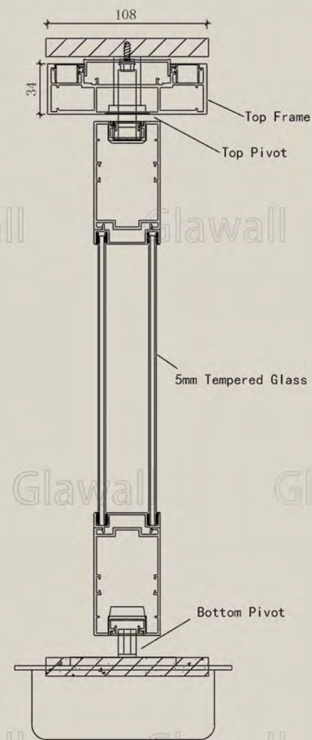
45 Series Pivot Door | Panel THK: 45mm
