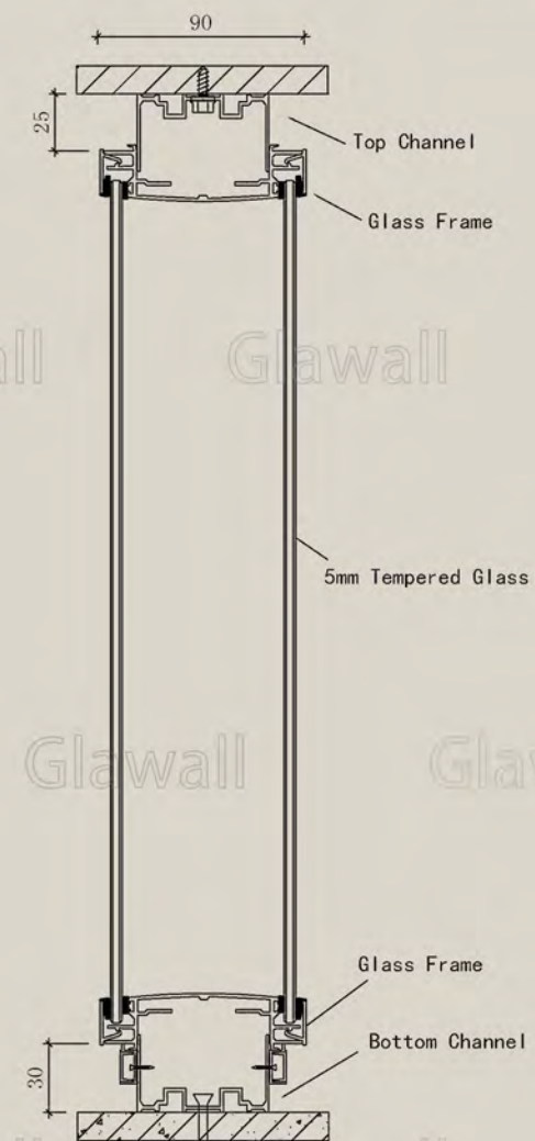
90 Series Double Glass Panel THK: 90mm
