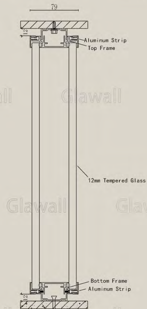
79 Series Frameless Double Glass | Panel THK: 79mm
