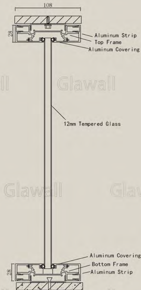
108 Series Frameless Single Glass | Panel THK: 108mm
