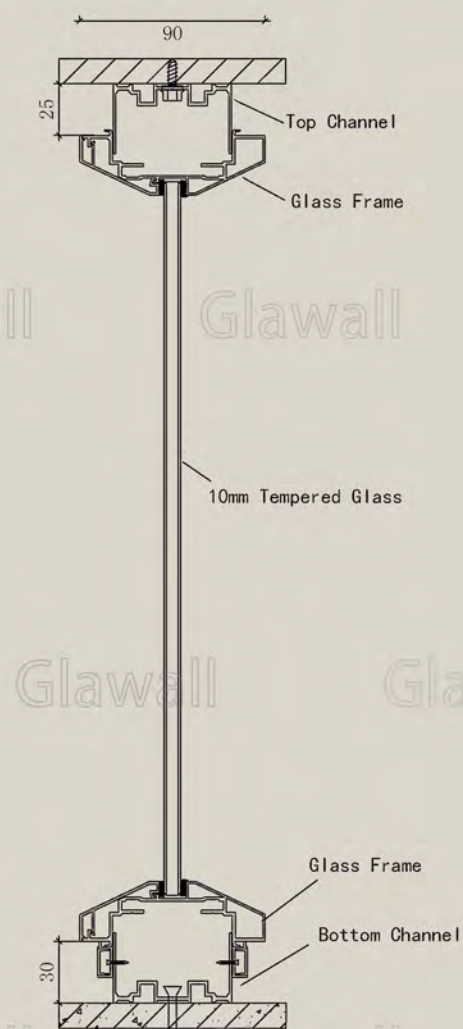
90 Series Single Glass Panel THK: 90mm
